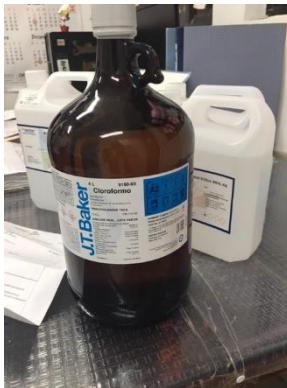
Clororformo
